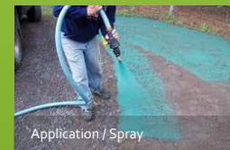
Hydromulch mixture (ready for application), includes; seedlings, Tacifier, Fertilizers, and microbial additives
